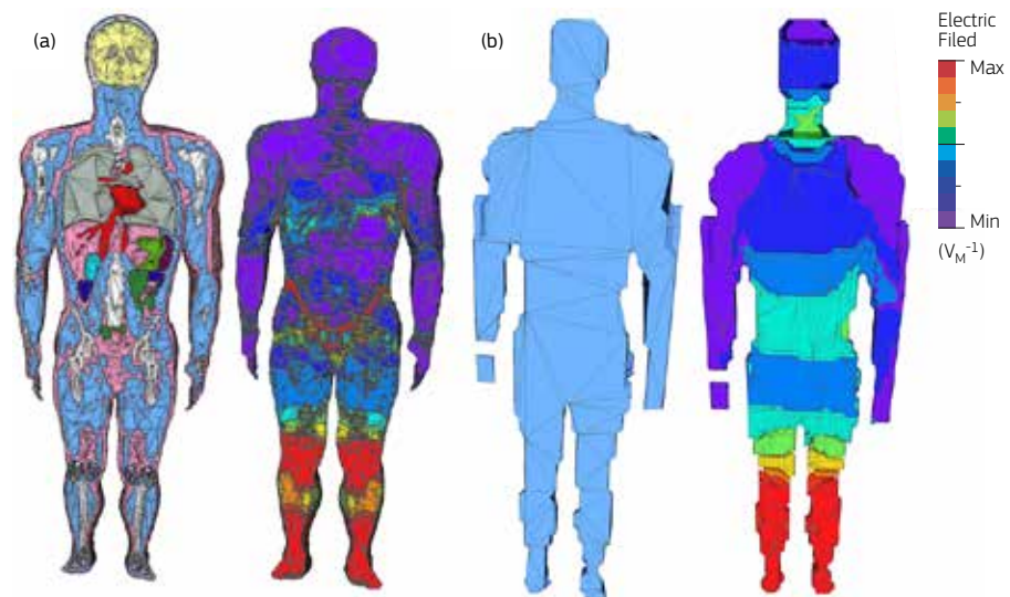
Figure D26 — Induced electric field distribution from exposure to a 50 Hz external electric field in (a) 2 mm resolution, high quality heterogeneous human model (b) 16 mm resolution, low quality homogeneous human model. Using low quality, low resolution homogeneous human models can introduce errors in the calculated values.
